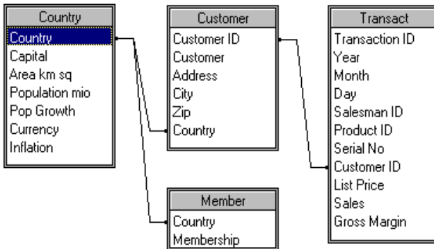
Figure 93. Four tables: a list of countries, a list of customers, a list of transactions and a list of memberships, which are associated with each other through the fields Country and CustomerID.
